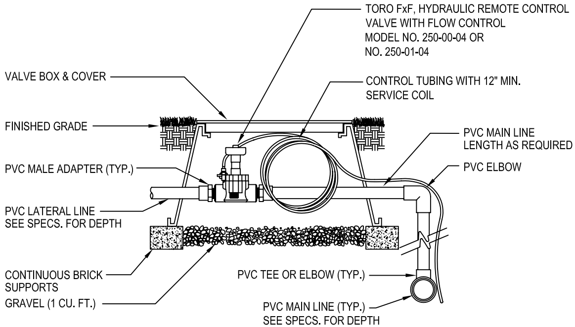
SECTION/ELEVATION NOT TO SCALE
